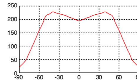
Compact Intensity Diagram 360W HPS
