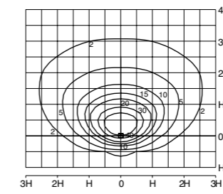
Compact Isolux Diagram 360W HPS, MT: 10M A: 68°
